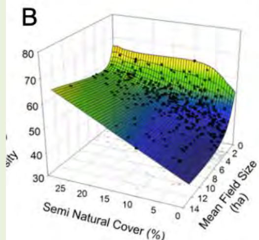
Figure. Relationship of field size and multi-taxa biodiversity index (y axis). Source: Sirami et al., 2019. 61
